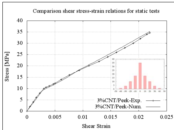
Fig. 6. Shear test results and CNT's
