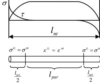
Fig. 3. Different regions in CNTs-interface.
