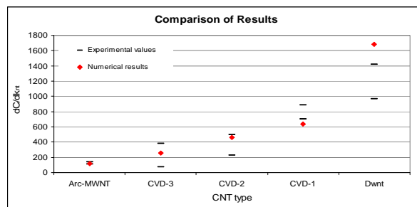
Fig. 4. Comparison of numerical and experimental results.
